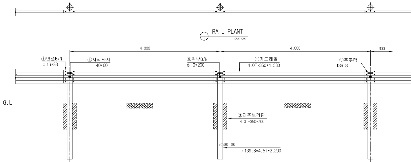
RAIL ELEVATION SCALE: NONE
