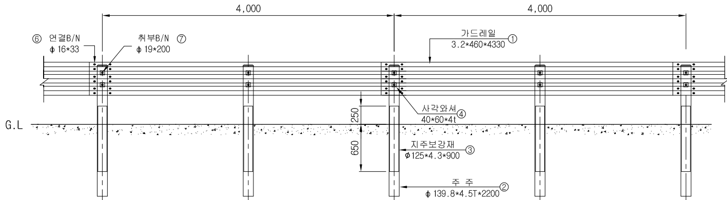
RAIL ELEVATION SCALE: NONE
