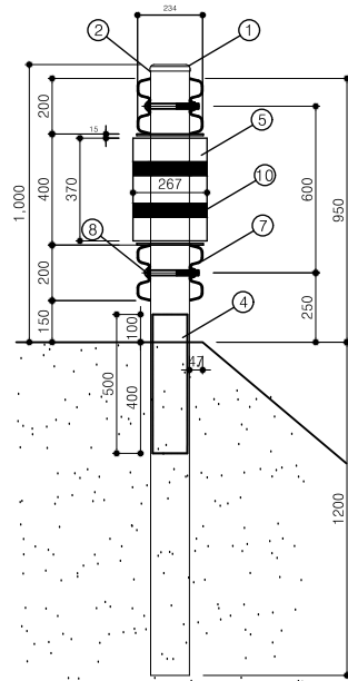
SIDE ELEVATION
