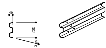
Detailed Rail
