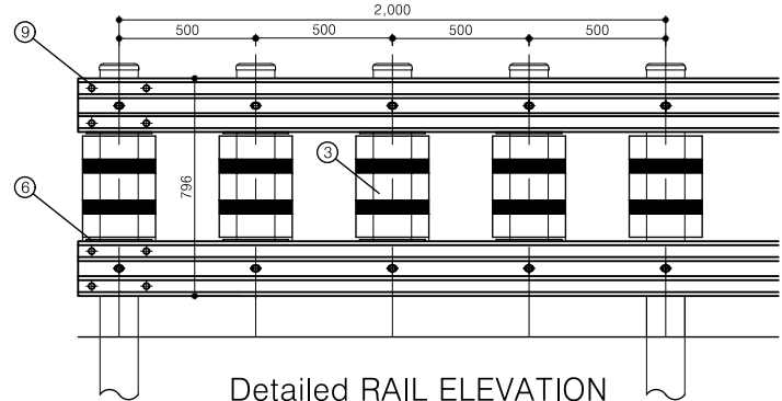
Detailed RAIL ELEVATION
