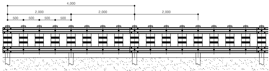
RAIL ELEVATION (S=1/2)
