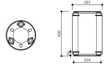
Detailed drawing of shock absorbing roller
