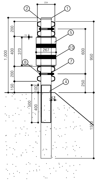
SIDE ELEVATION
