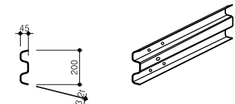
Detailed Rail
