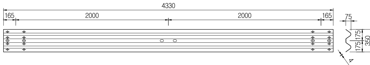
Guard Rail SCALE : NONE
