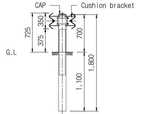
SIDE ELEVATION SCALE : NONE
