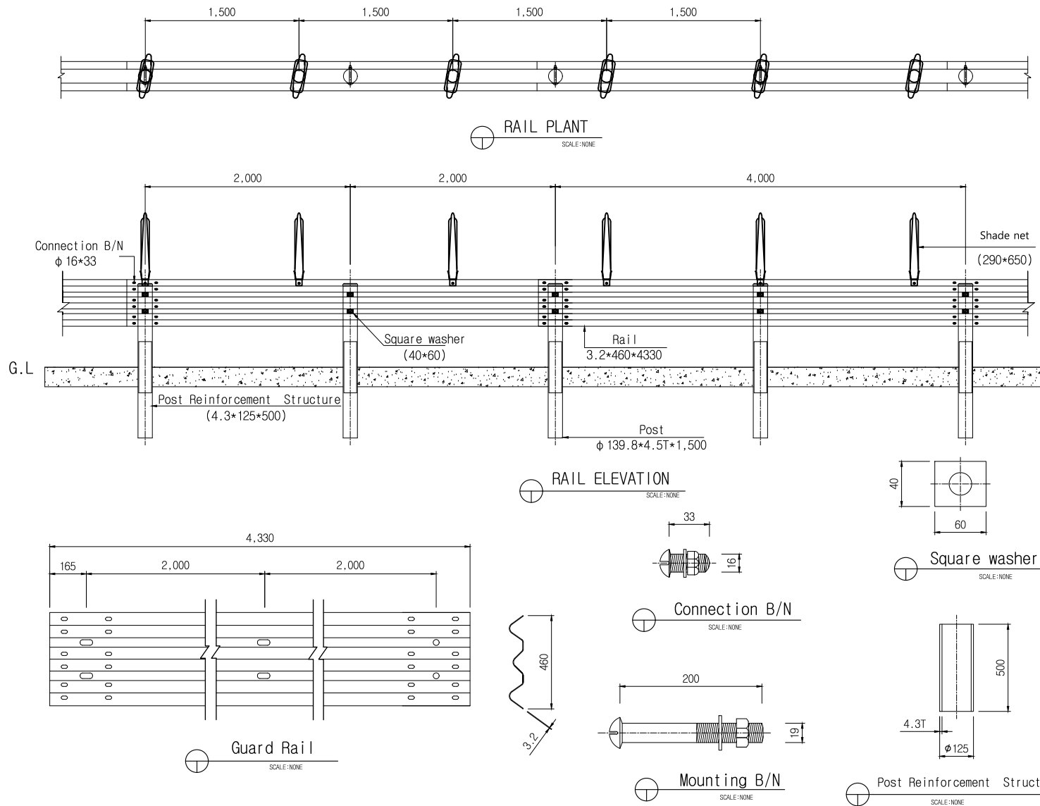
Standard Section(Per span)
