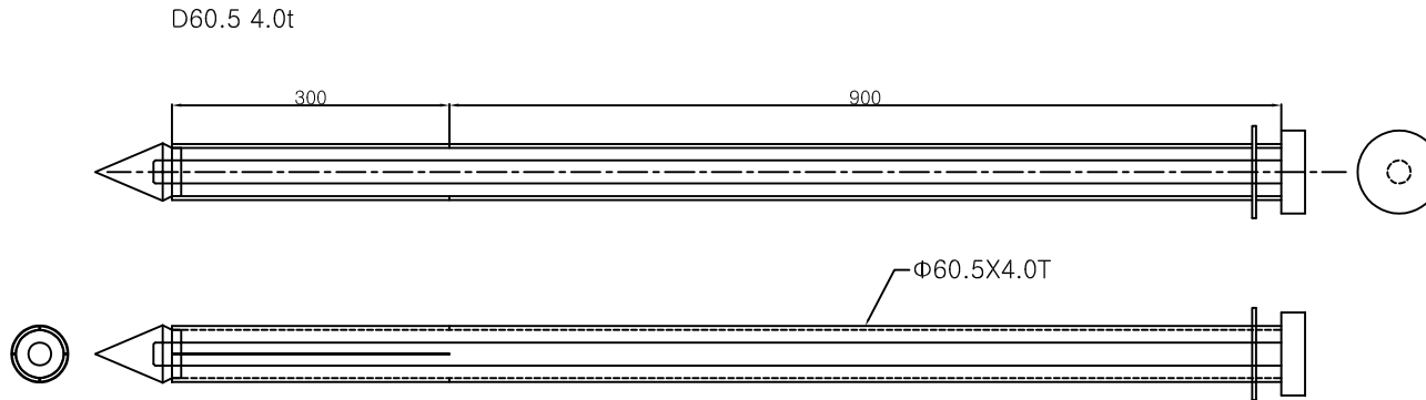
Anchor assembly
