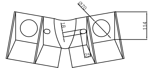
Bracket detailed drawing
