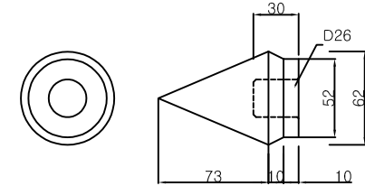
wedge detail
