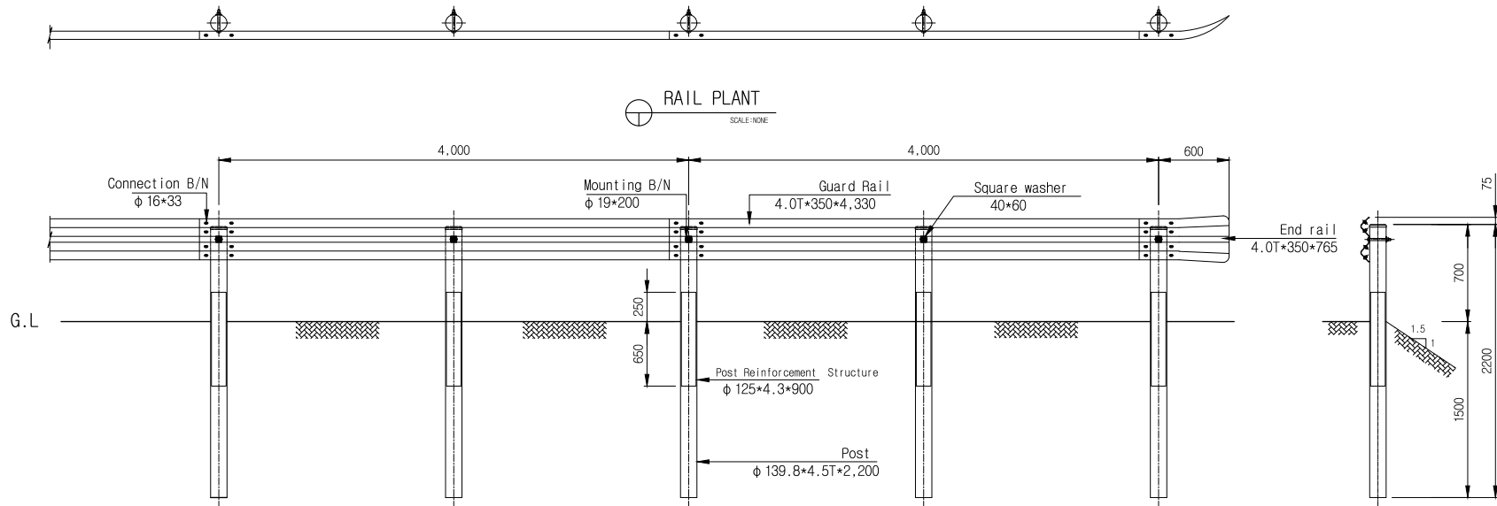
RAIL ELEVATION SCALE: NONE
