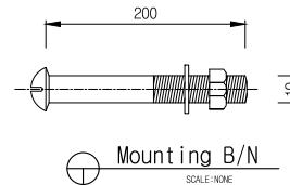
Connection B/N SCALE: NONE
